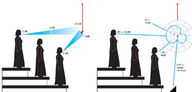
Side view: The first choir rows are closer to the microphone than the back rows. Angling the hypercardioid pattern creates a balanced sound.
